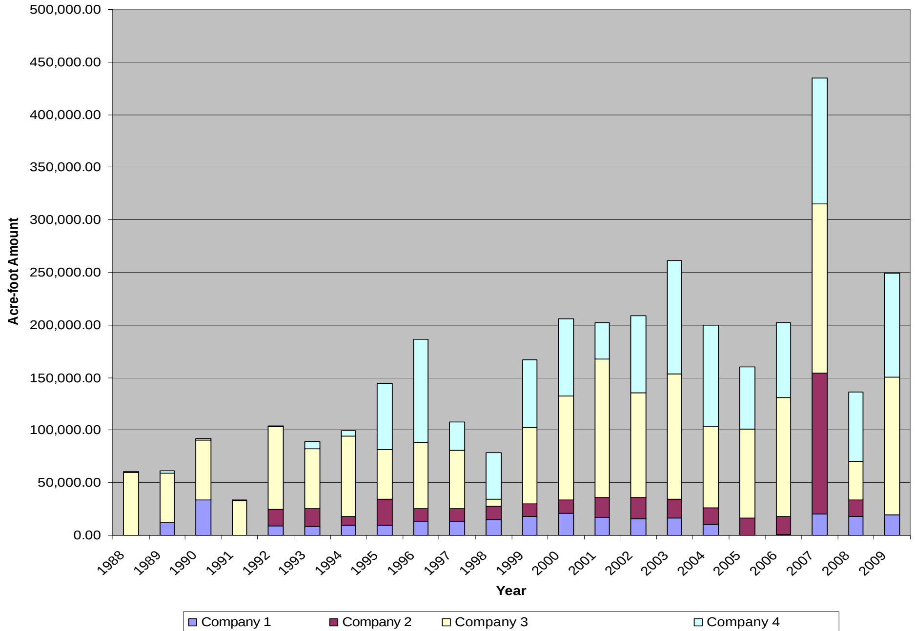
Water Pumped from the Great Salt Lake
