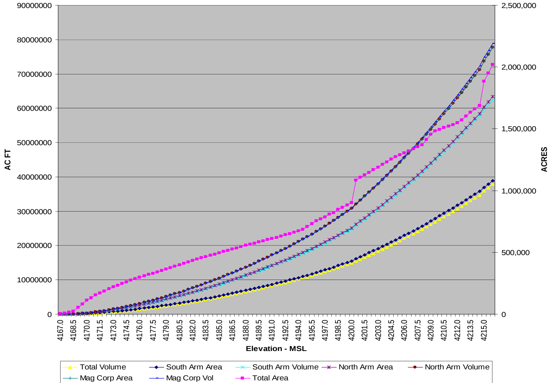
GSL Area Volume Curves
